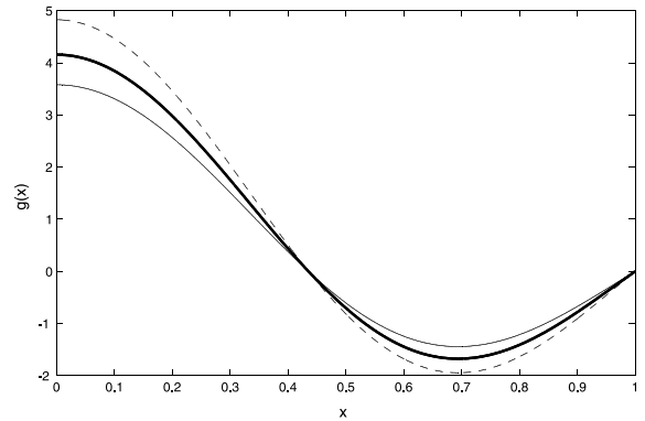
Fig. 2. The case m = 2, T = 1, \epsilon = 0.004 .
