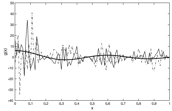
Fig. 7. The case of noisy data with SNR = 1160 dB, N = 4 , T = 1 , m = 4 , \epsilon = 0.002 .
