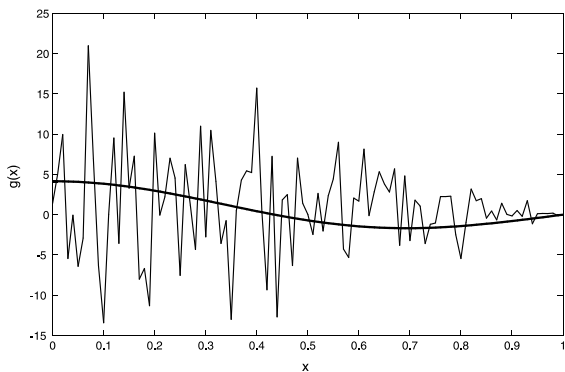
Fig. 11. The case of noisy data with SNR = 30 dB, N = 3 , T = 2 , m = 2 , \epsilon = 0.1 .
